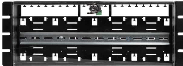
Sheet metal housing with DIN rail for 19" rack or mounting directly on the wall, the product comes with a tamper switch.
