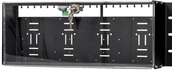
Sheet metal housing for 19" rack or mounting directly on the wall, the product comes with a tamper switch. 19 rack DIN module holder
