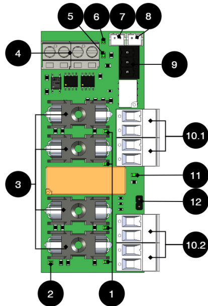
Circuit Board Overview - 2+2 Output module
